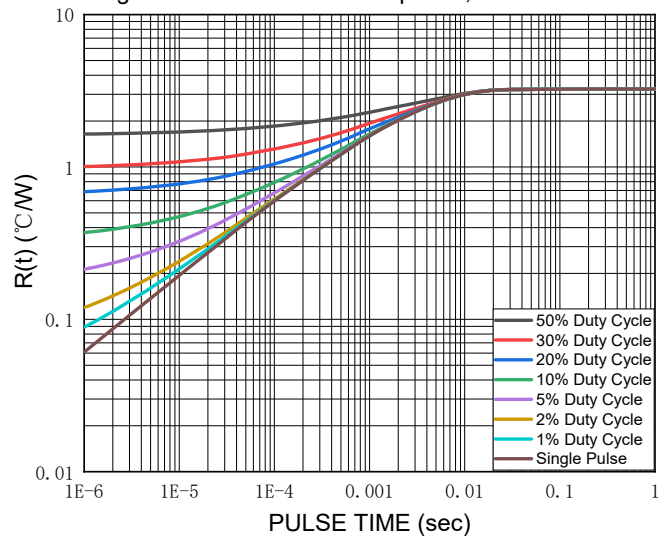
Fig.6: Transient Thermal Response, Junction to Case
